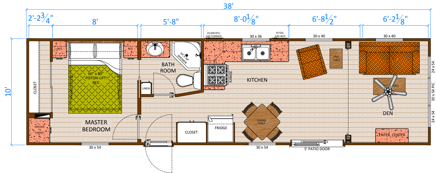
IMPERIAL (I3810 DEN) FLOOR PLAN (380 SQ.FT.)
