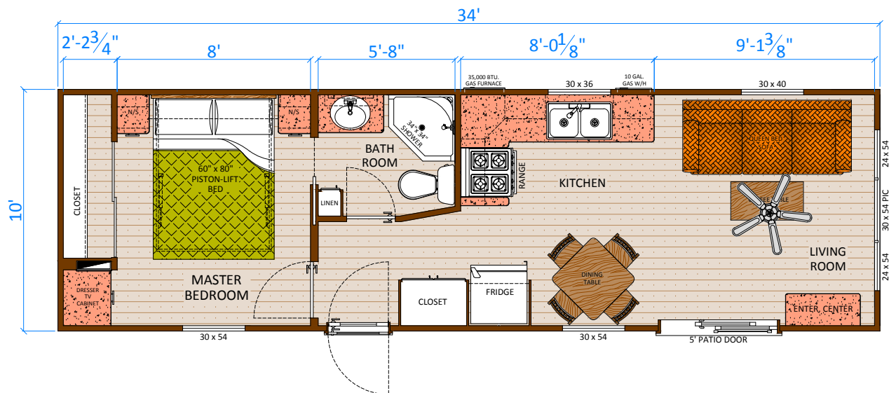
INGLESIDE (I3410 FL) FLOOR PLAN (340 SQ.FT.)
