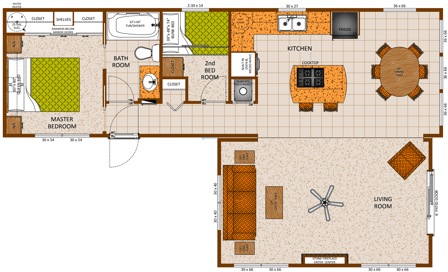
RESOLUTE - (R4124) (492 SQ.FT.)+(240 SQ.FT.)
